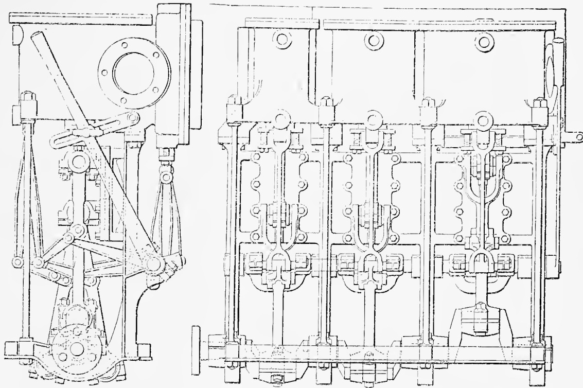
TRIPLE-EXPANSION ENGINE OF 36-FOOT STEAM LAUNCH WILD DUCK.
